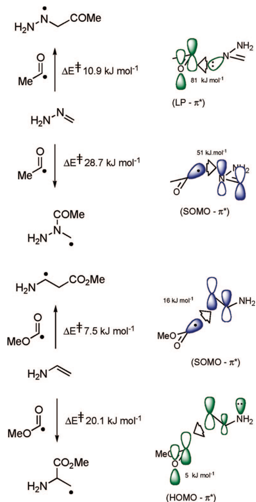
FIGURE 16. Examples of “dual orbital” interactions in reactions involving acyl and oxyacyl radicals. Energies calculated at the BHandHLYP/6-311G** level of theory.
